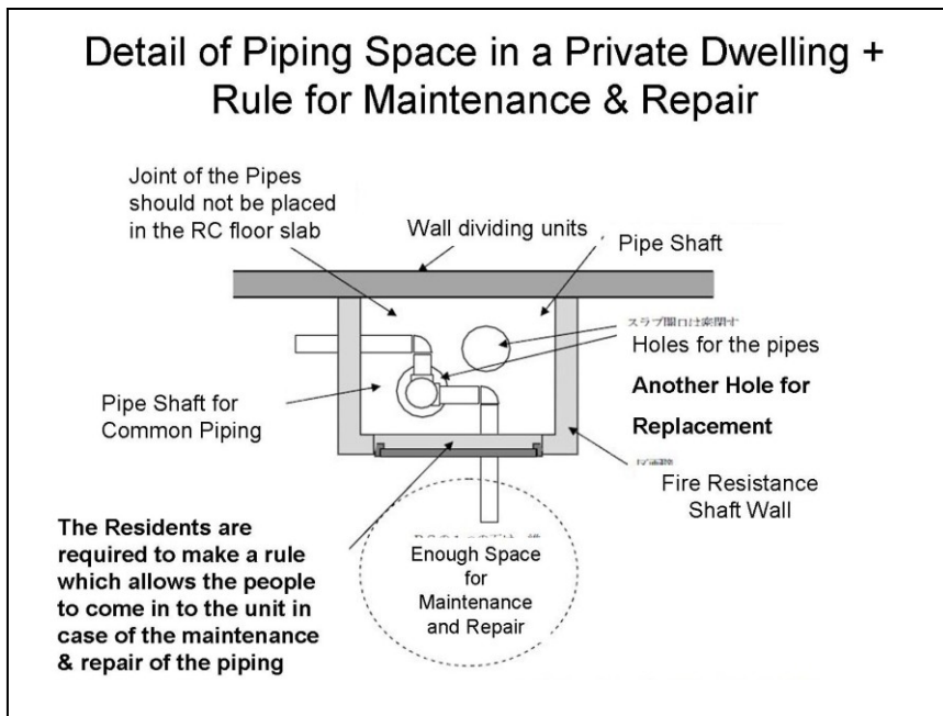
Figure 1. The requirements for piping space in a private condominium dwelling
