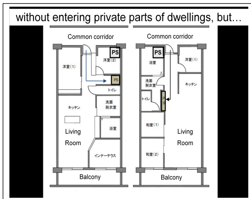
Figure 2. The common piping of condominium apartments that can be maintained without entering private parts of dwellings.
